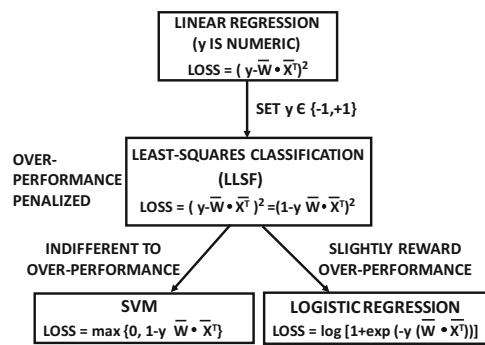
(b) Relationships among linear models
