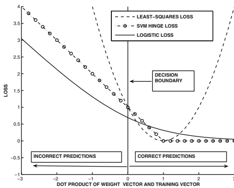
(a) Loss functions of optimization models
